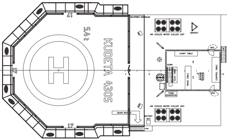
HELIDECK PLAN / 04 DECK
