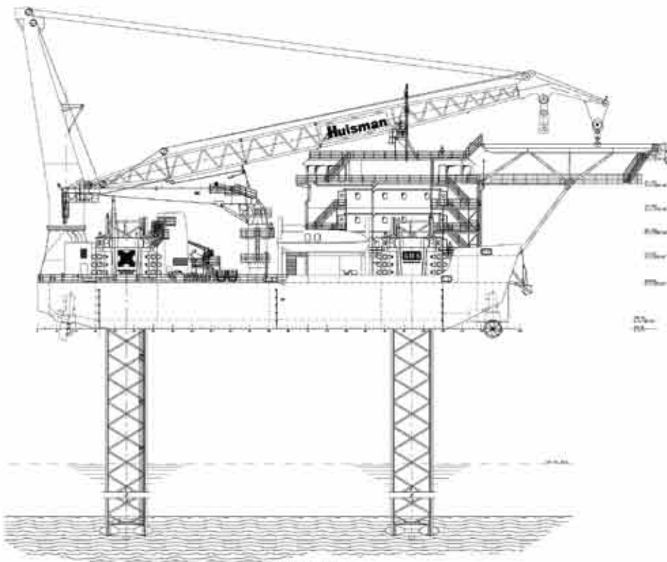
OUTBOARDPROFILE
