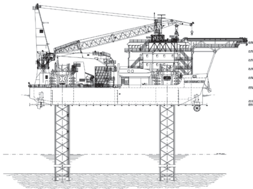
OUTBOARD PROFILE
